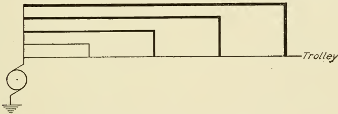
Fig. 208. Diagram of Trolley Feeder System
